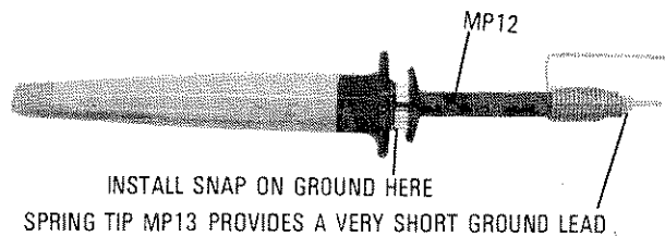
Figure 2. Probe with Ground Spring
