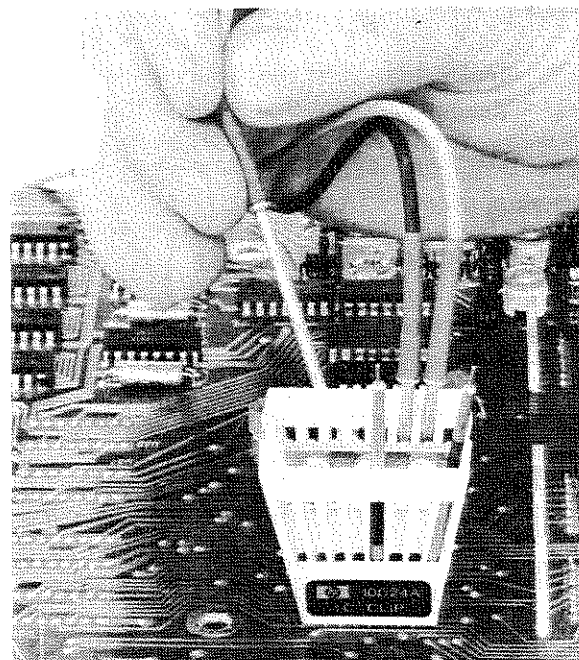
Figure 4. Use of Probe with Model 10024A IC Test Clip
