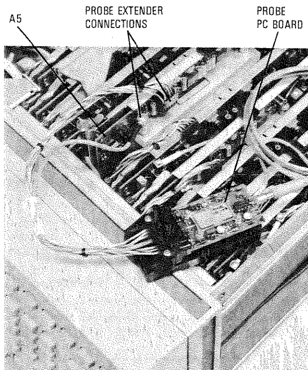
Figure 6. Probe Extender Connections
