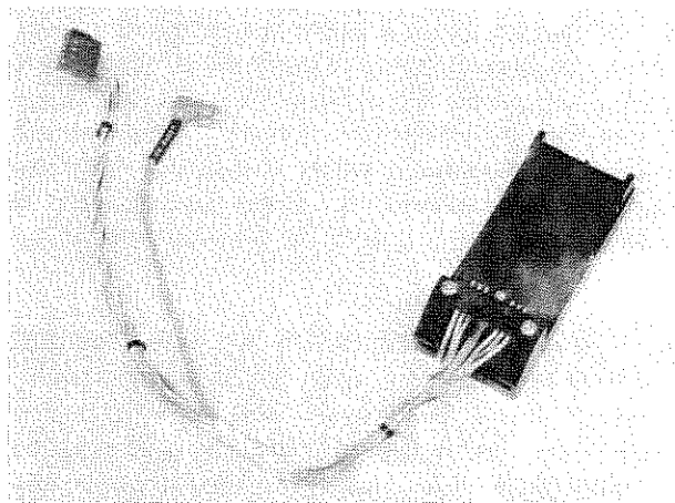
Figure 5. Probe Extender HP Part No. 54100-63802
