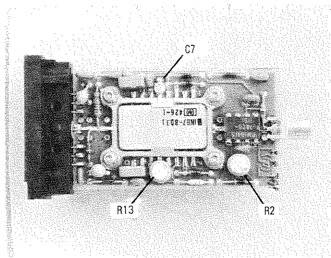
Figure 8. Probe PC Board
